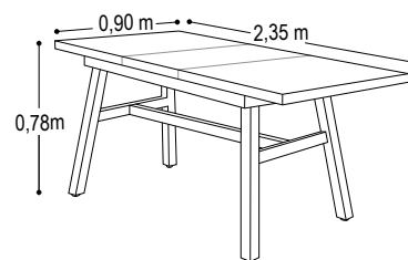
Mesa expandida
