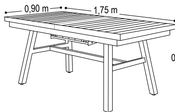
Mesa cerrada
